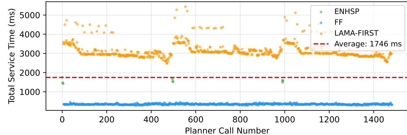
Planning Latency Per Call (LAMA-First + Metric-FF)
