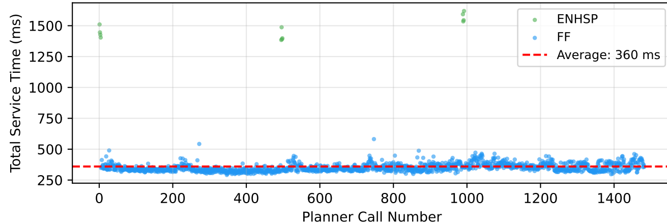
Planning Latency Per Call (Metric-FF)
